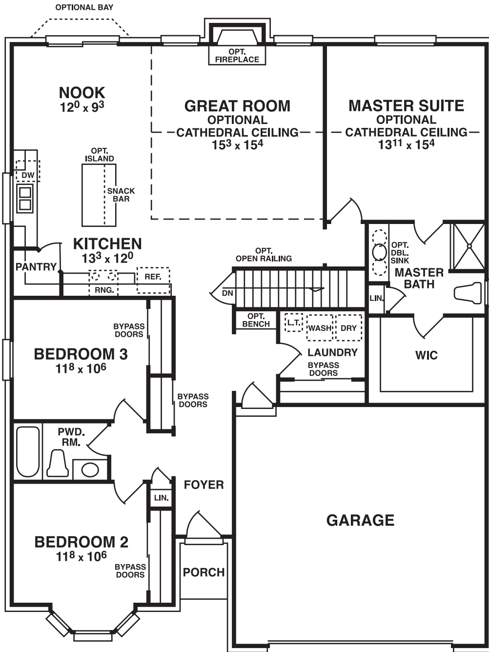
FIRST FLOOR PLAN ELEVATION B
