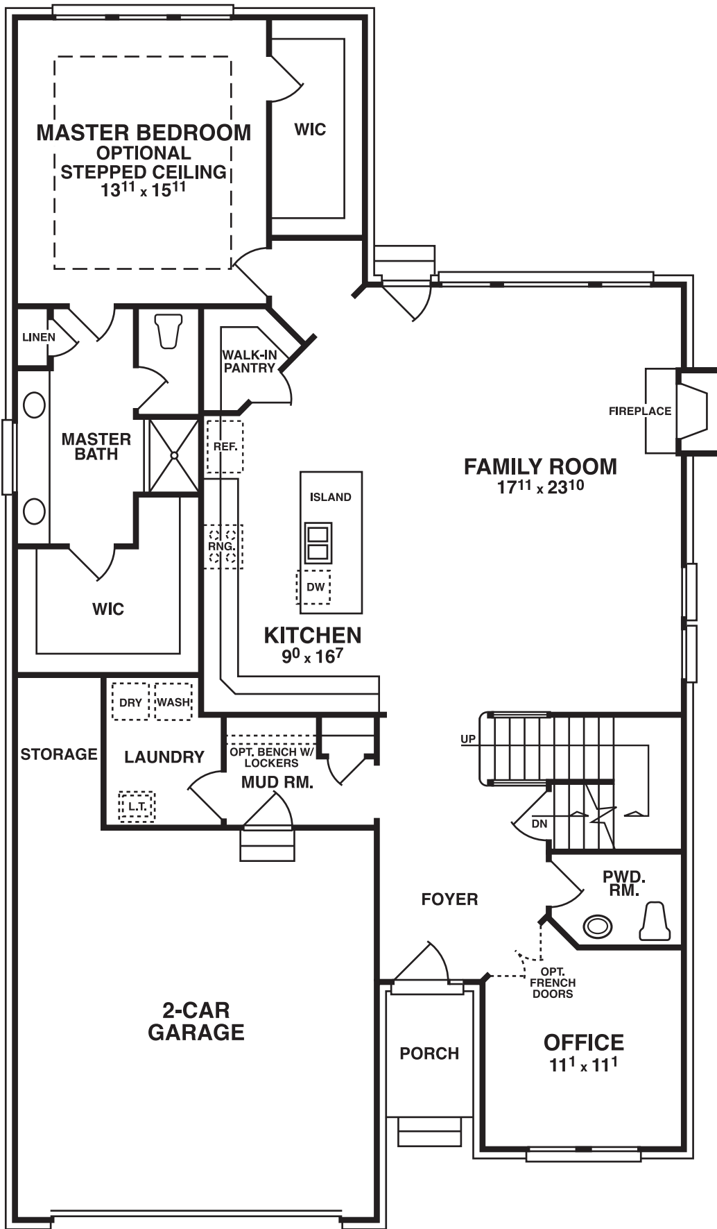
FIRST FLOOR PLAN ELEVATION A
