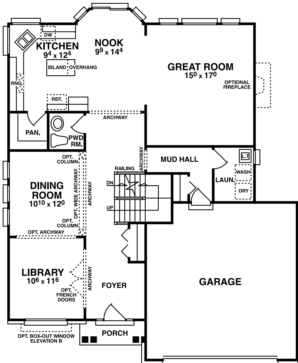
FIRST FLOOR PLAN ELEVATION A
