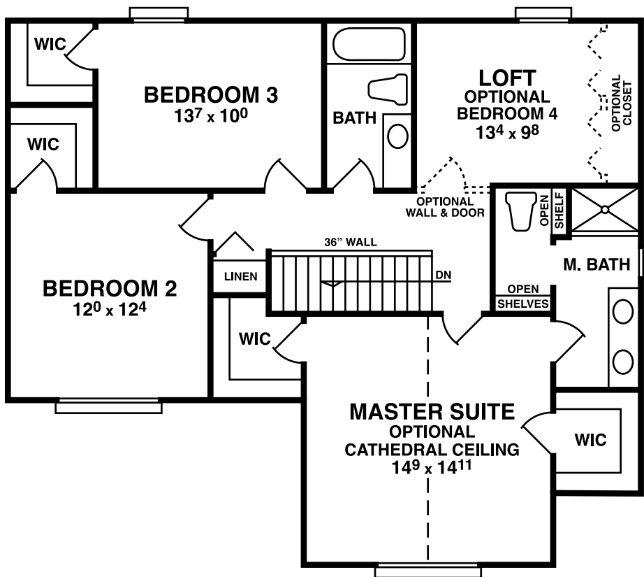
SECOND FLOOR PLAN ELEVATION A
