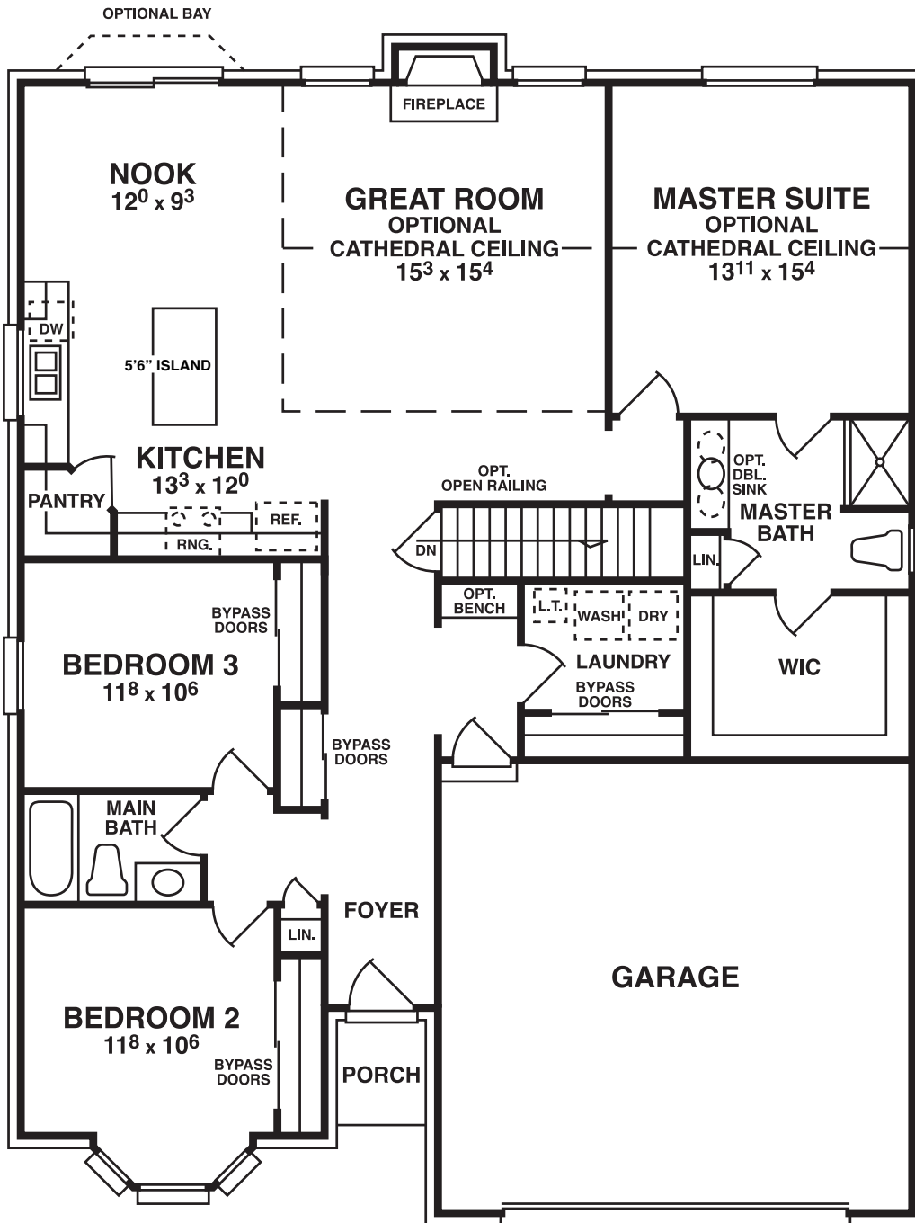
FIRST FLOOR PLAN ELEVATION B
