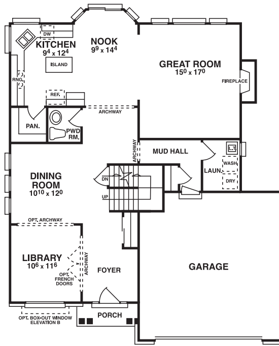
FIRST FLOOR PLAN ELEVATION A
