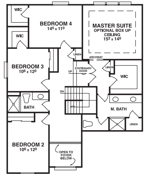
SECOND FLOOR PLAN ELEVATION A
