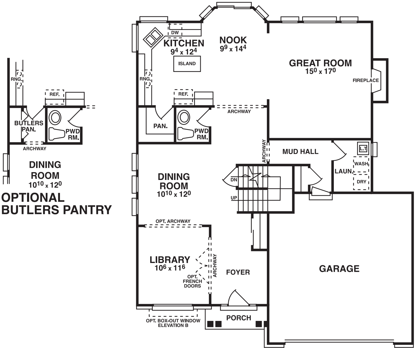
FIRST FLOOR PLAN ELEVATION A
