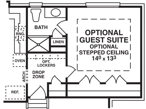
OPTIONAL GUEST SUITE PLAN
