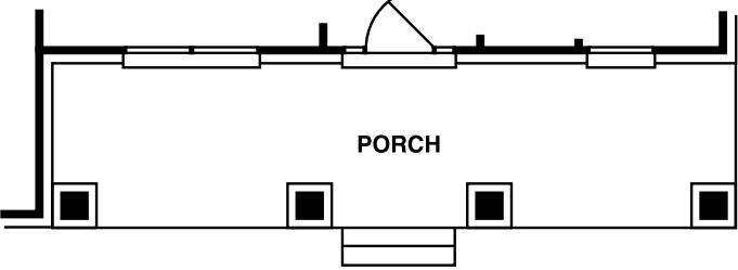
PORCH PLAN ELEVATION B
