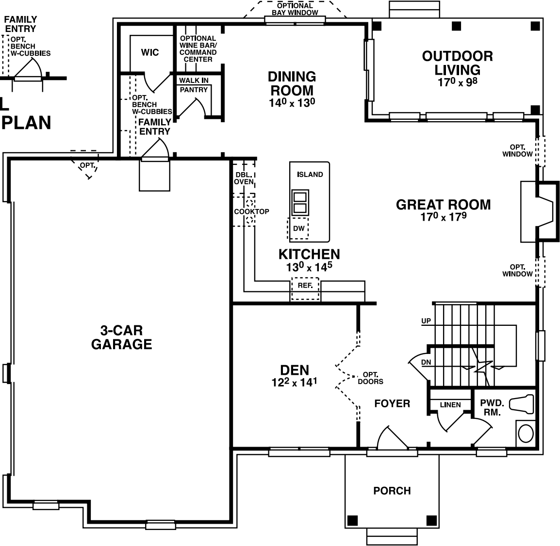
FIRST FLOOR PLAN ELEVATION A
