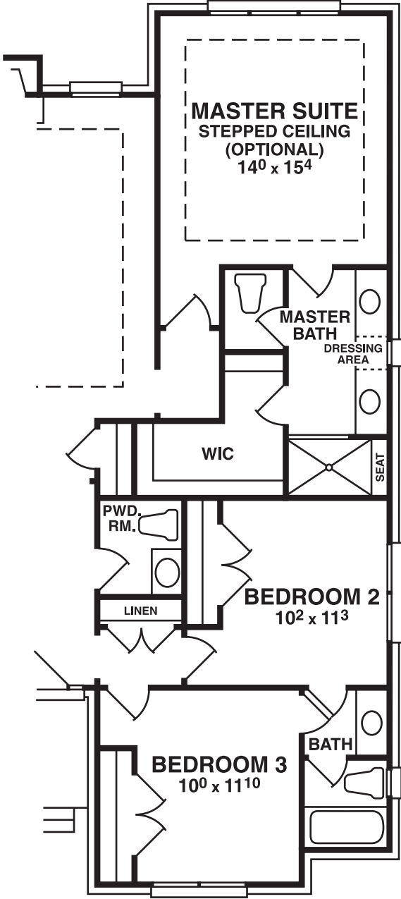
OPTIONAL 3 BEDROOM PLAN ELEVATION A
